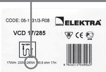
Self-adhesive label
